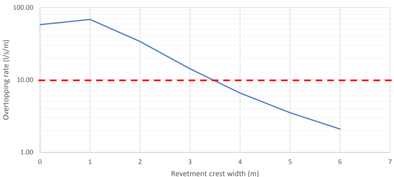
Optimisation of the revetment crest width (1 in 200-year)
