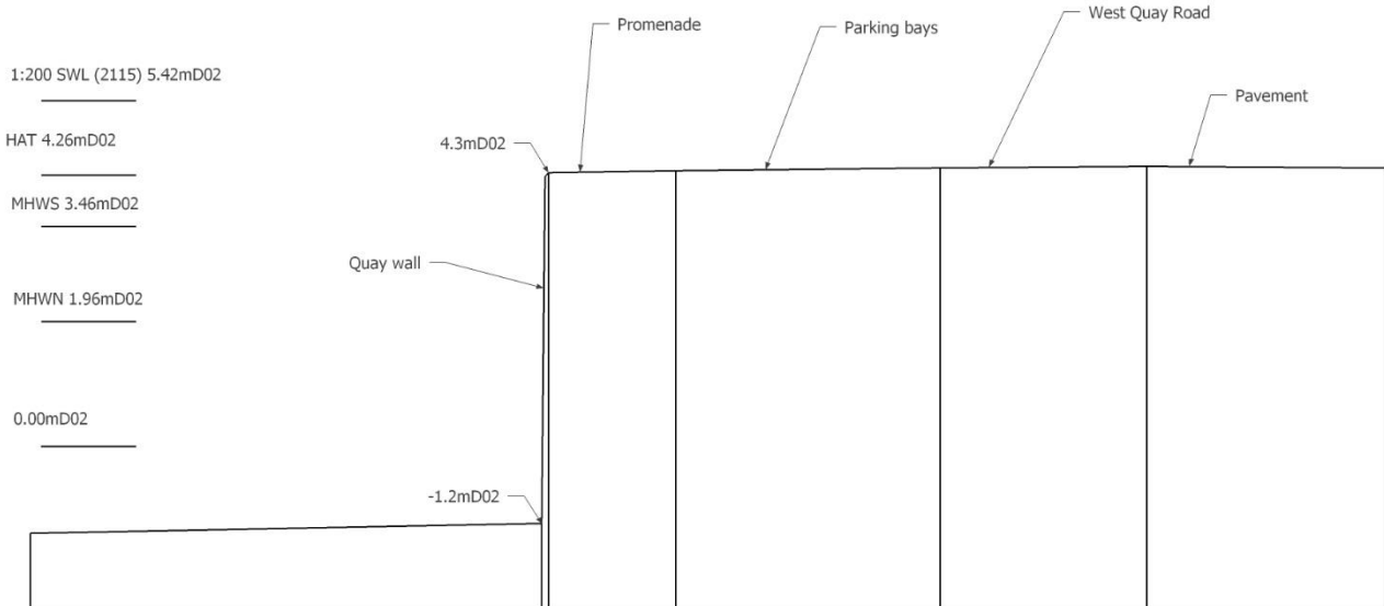
Figure 2-1: Existing section through Ramsey Harbour
