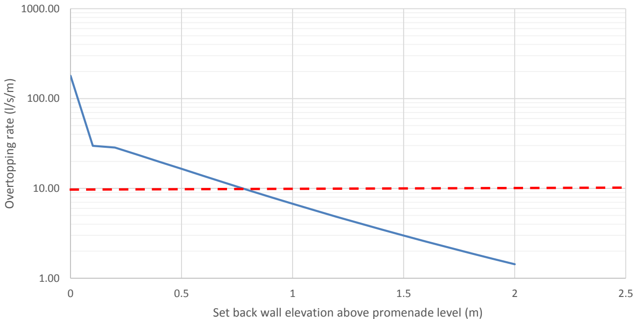
Optimisation of set back wall elevation (1 in 200-year)
