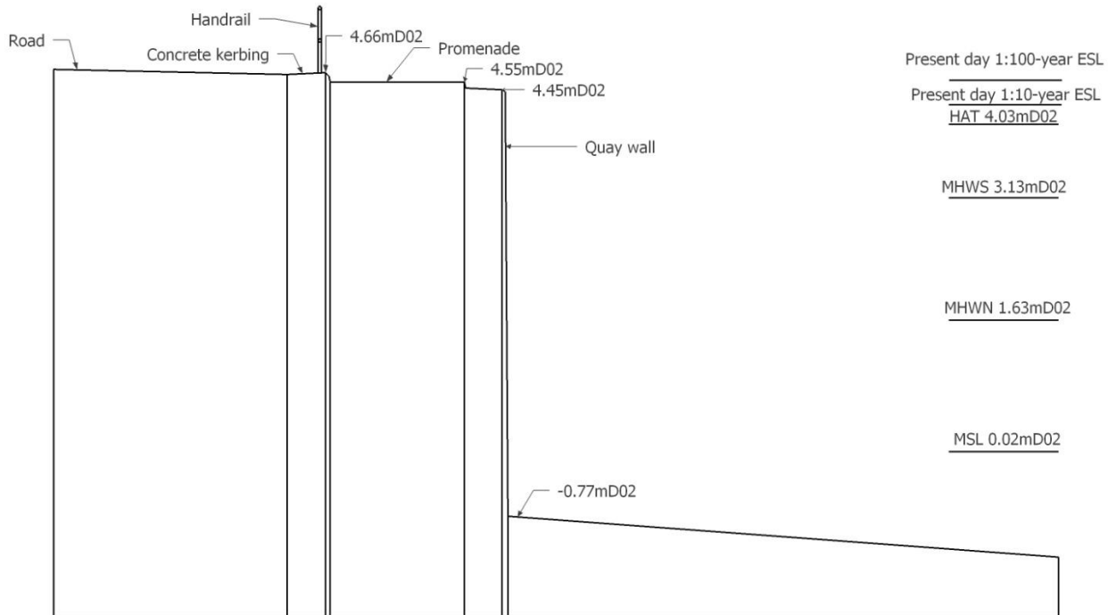
Figure 2-1: Existing section through Douglas Harbour
