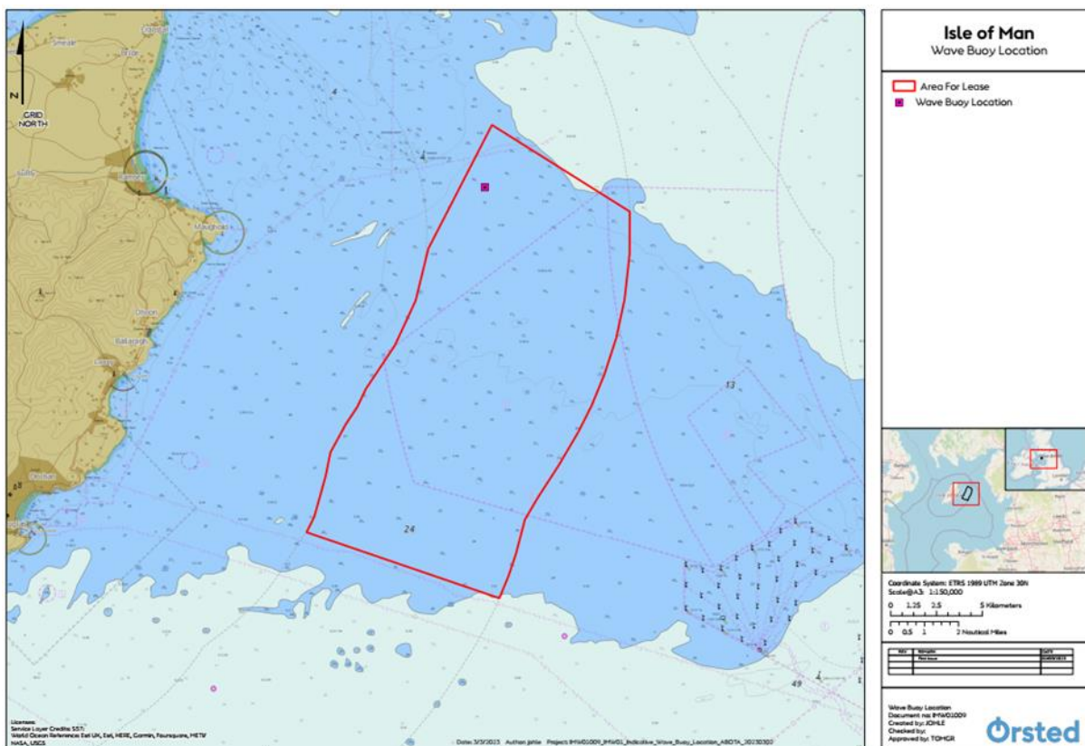
Figure 1 – Buoy Location.
